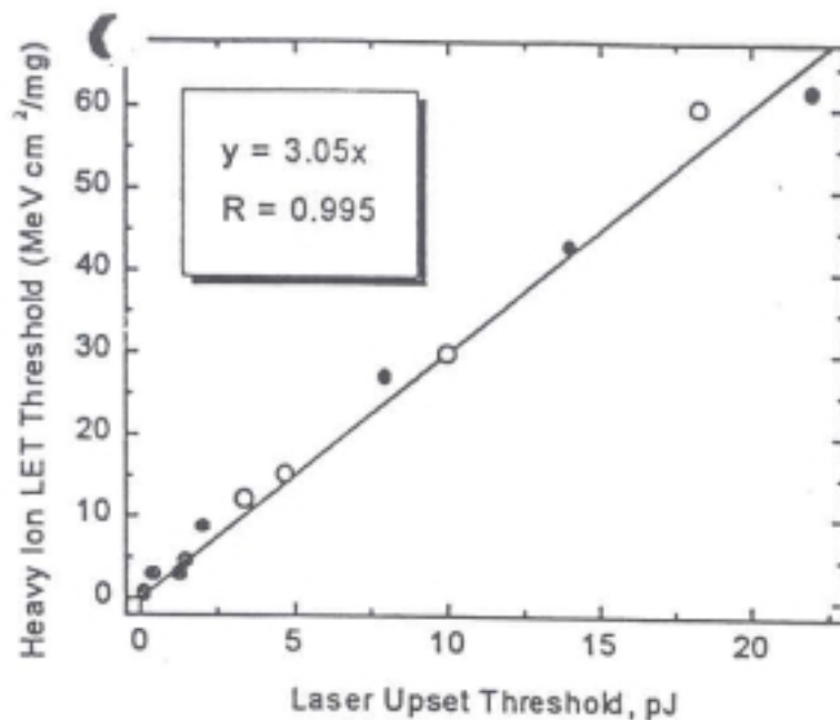
Figure 5. Measured heavy ion SEU and SEL LET thresholds plotted against the measured laser upset threshold for data for 13 cases listed in Table 3.
